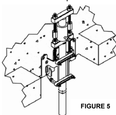
Typical Installation of Foundation Repair Brackets
